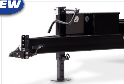
New Standard Adjustable Coupler/HD 12K Dropleg Jack
